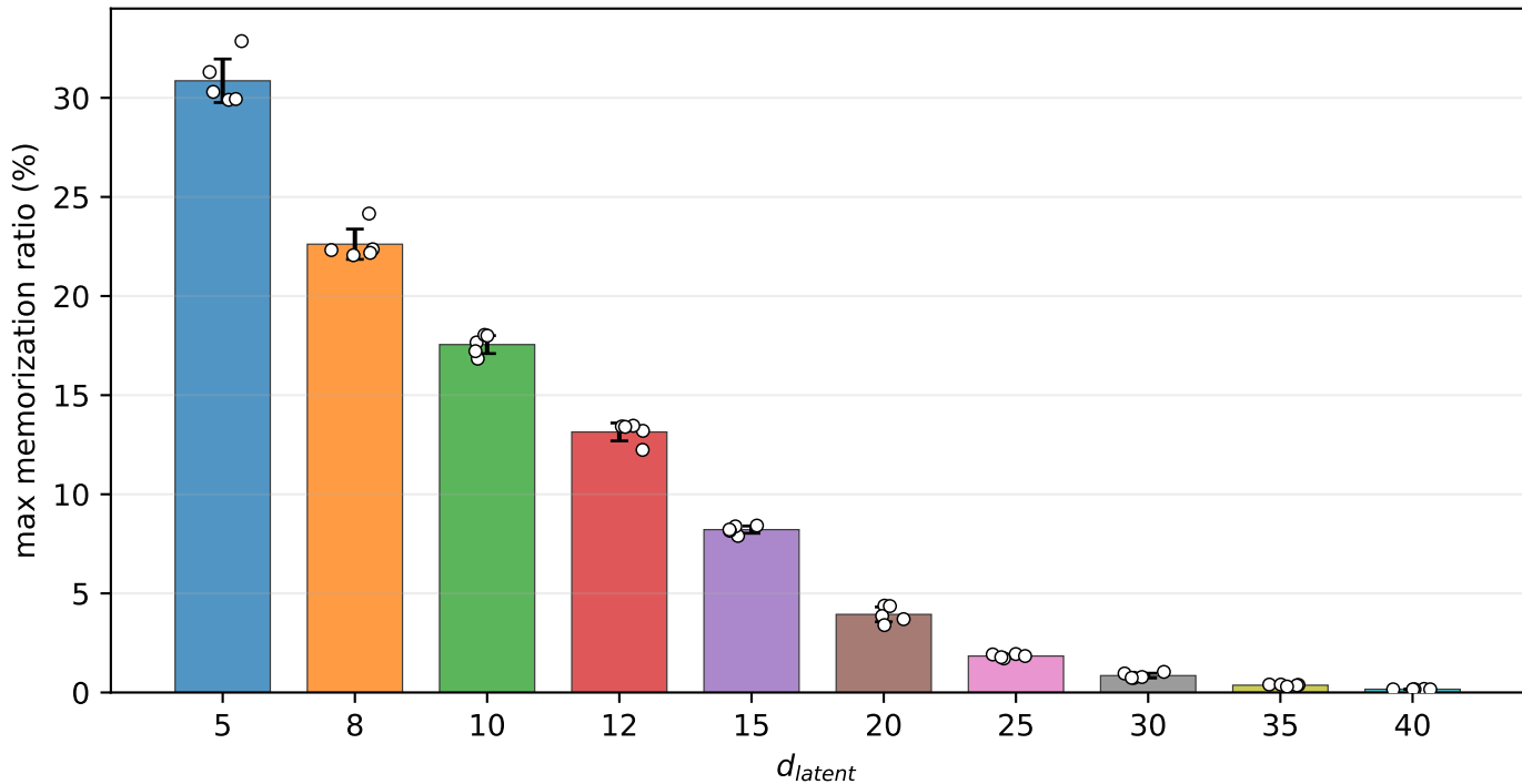
Maximum memorization ratio across training, 5-seed mean
